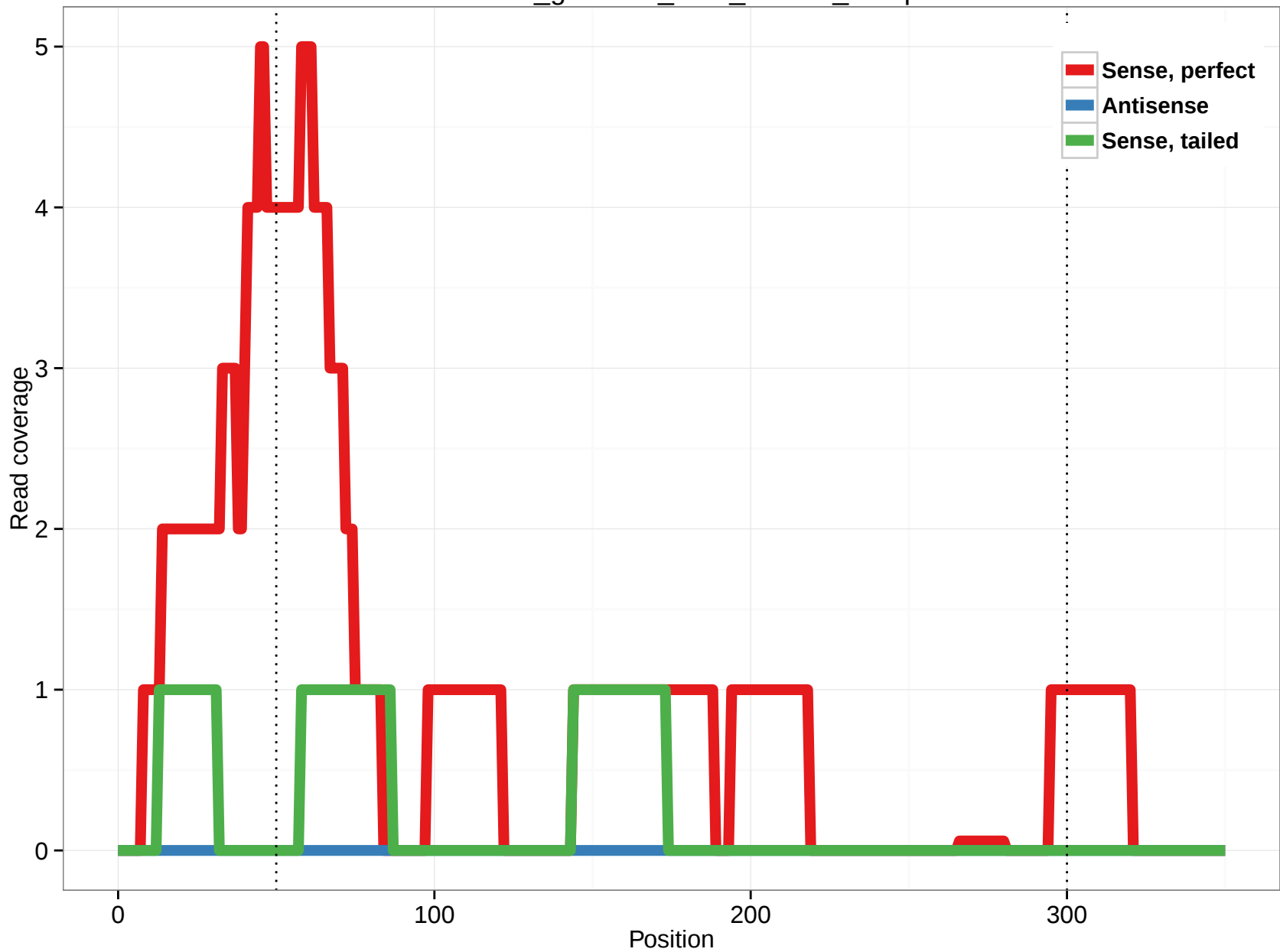
rheMac3_genscan_chr8_165.12_11.5p
