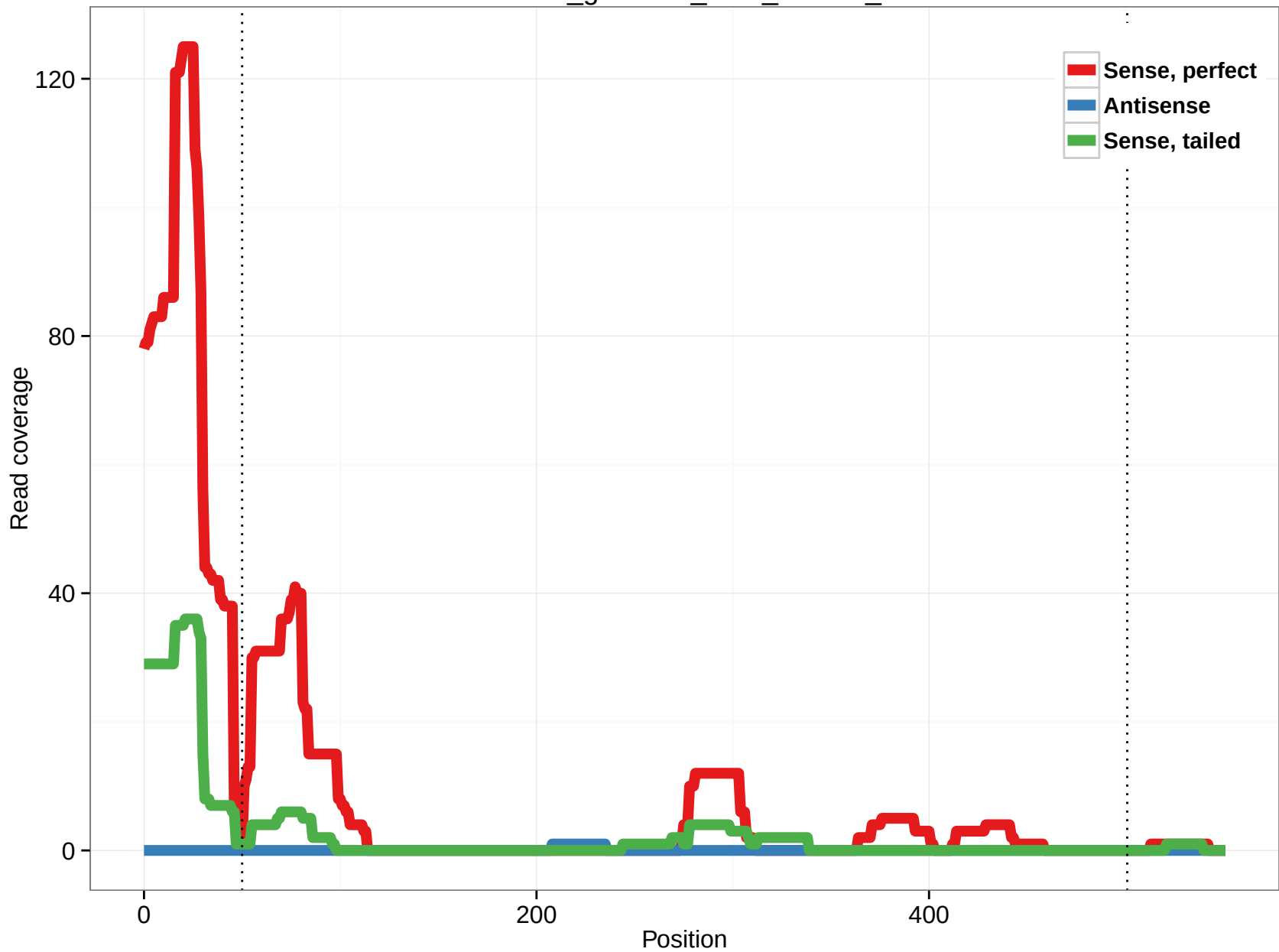
rheMac3_genscan_chr8_163.36_35
