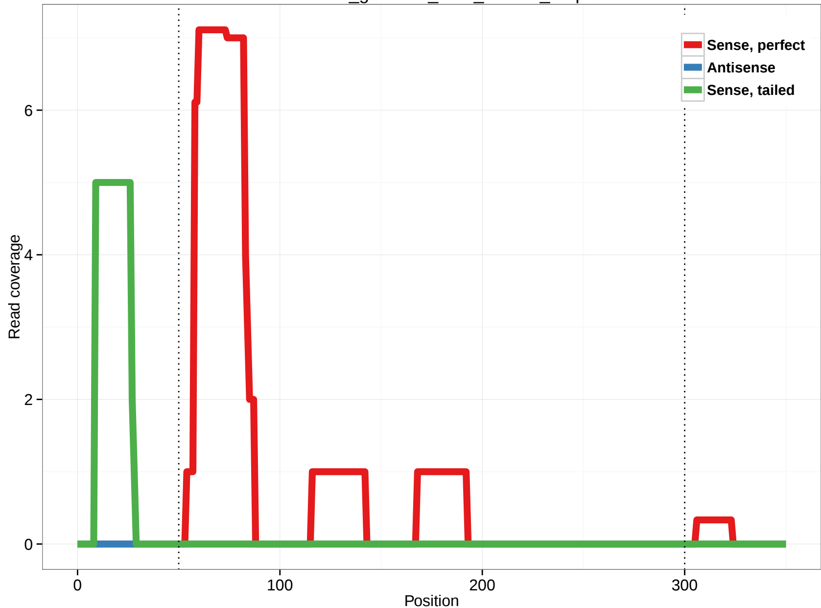
rheMac3_genscan_chr8_163.35_6.3p
