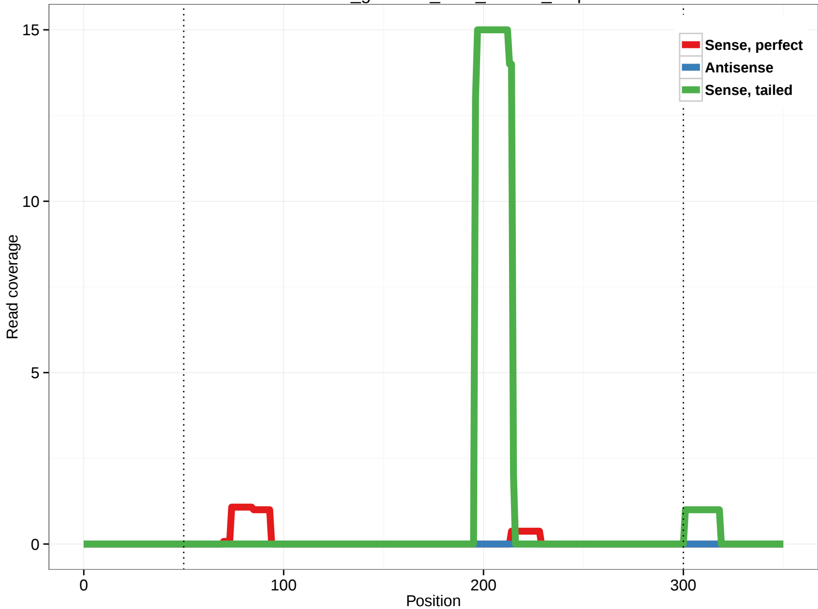
rheMac3_genscan_chr8_163.32_2.5p
