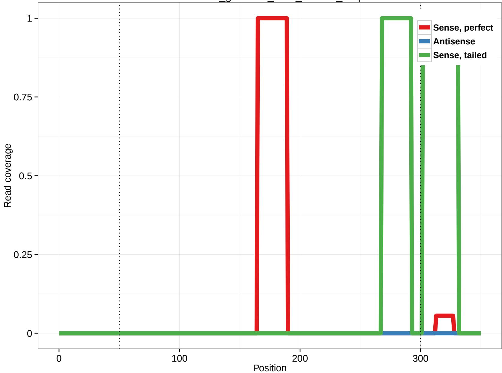
rheMac3_genscan_chr8_163.27_0.3p
