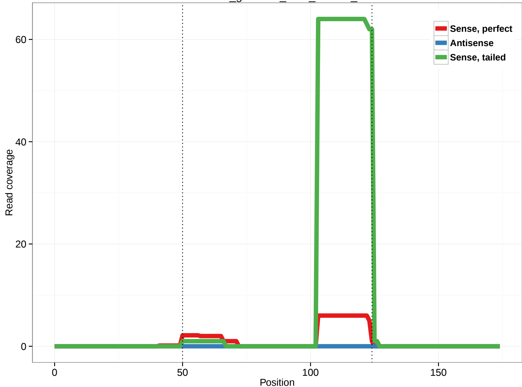
rheMac3_genscan_chr8_163.25_39
