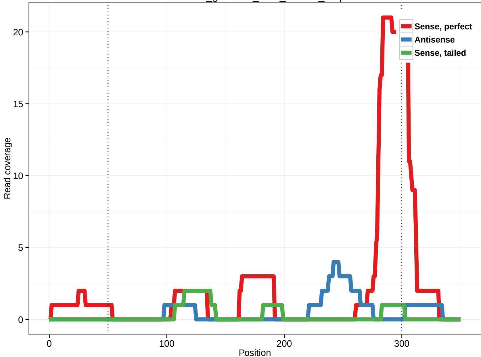
rheMac3_genscan_chr8_162.54_0.5p
