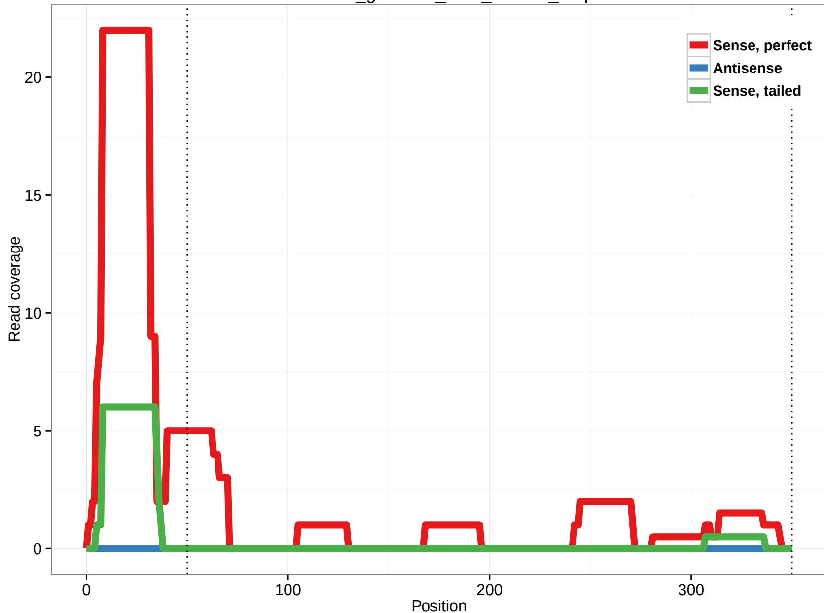
rheMac3_genscan_chr8_160.52_4.5p
