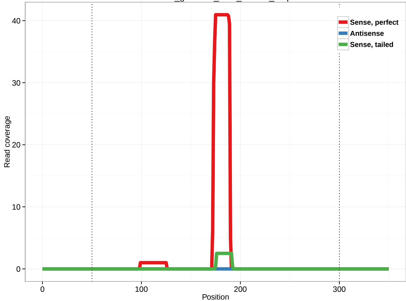
rheMac3_genscan_chr8_160.38_5.5p
