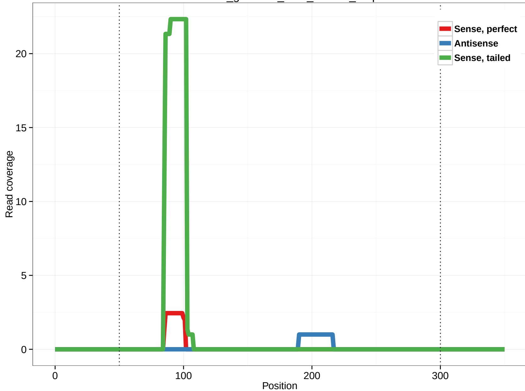
rheMac3_genscan_chr8_160.19_7.5p
