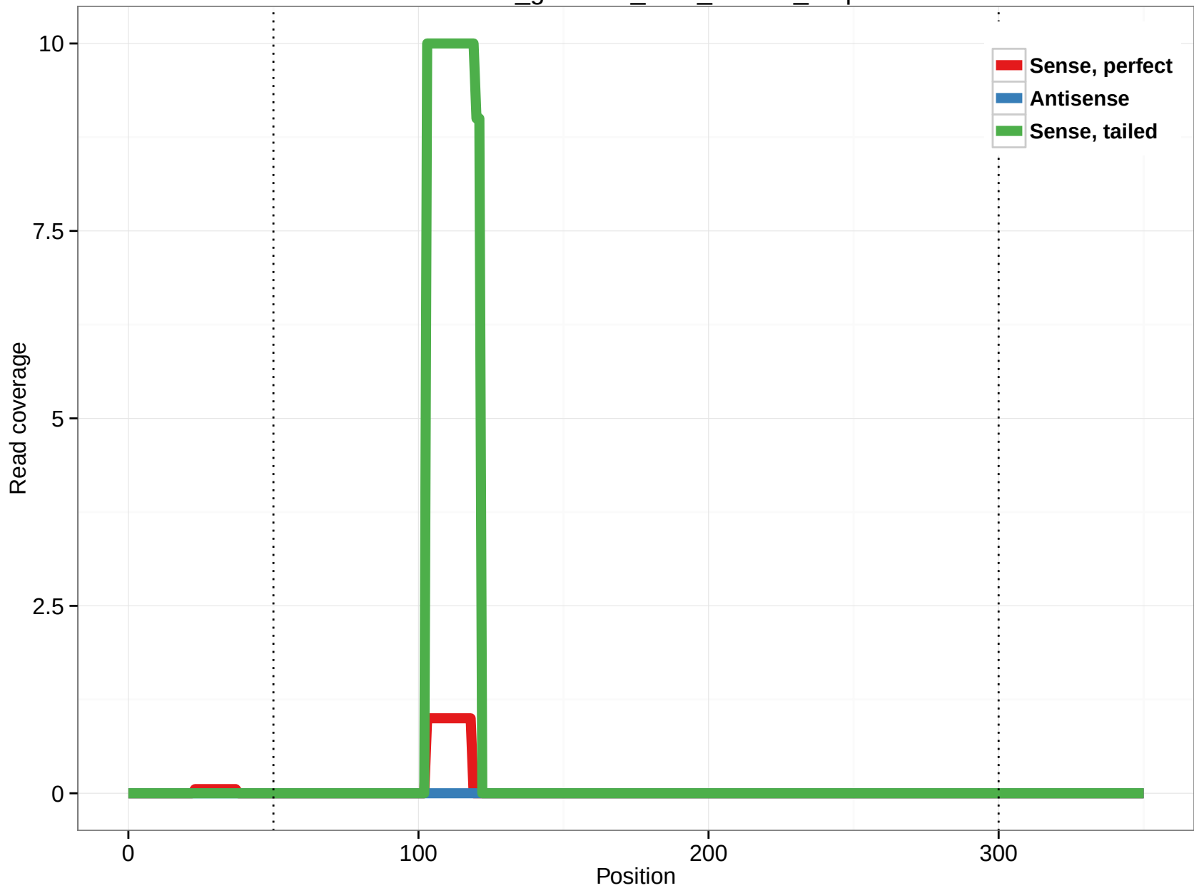
rheMac3_genscan_chr8_155.93_0.5p
