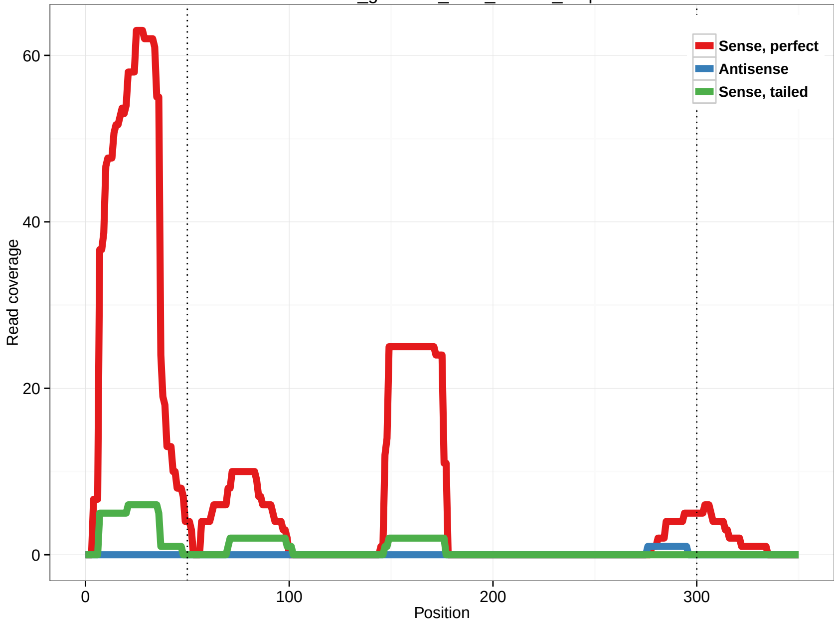
rheMac3_genscan_chr8_155.84_2.5p
