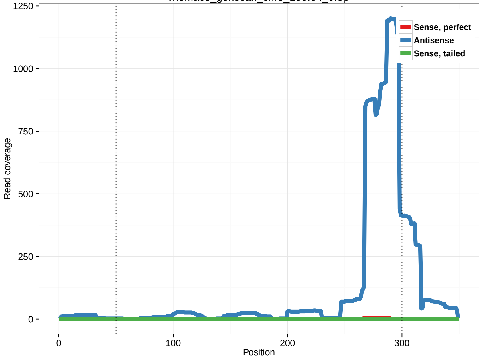
rheMac3_genscan_chr8_155.84_0.3p
