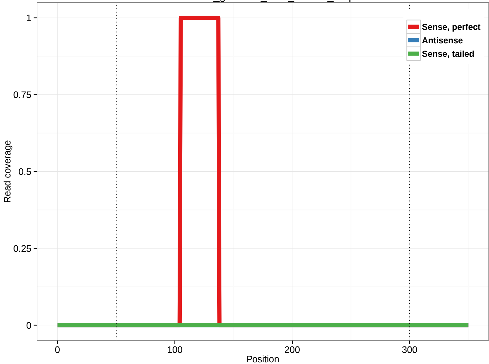
rheMac3_genscan_chr8_155.72_1.5p
