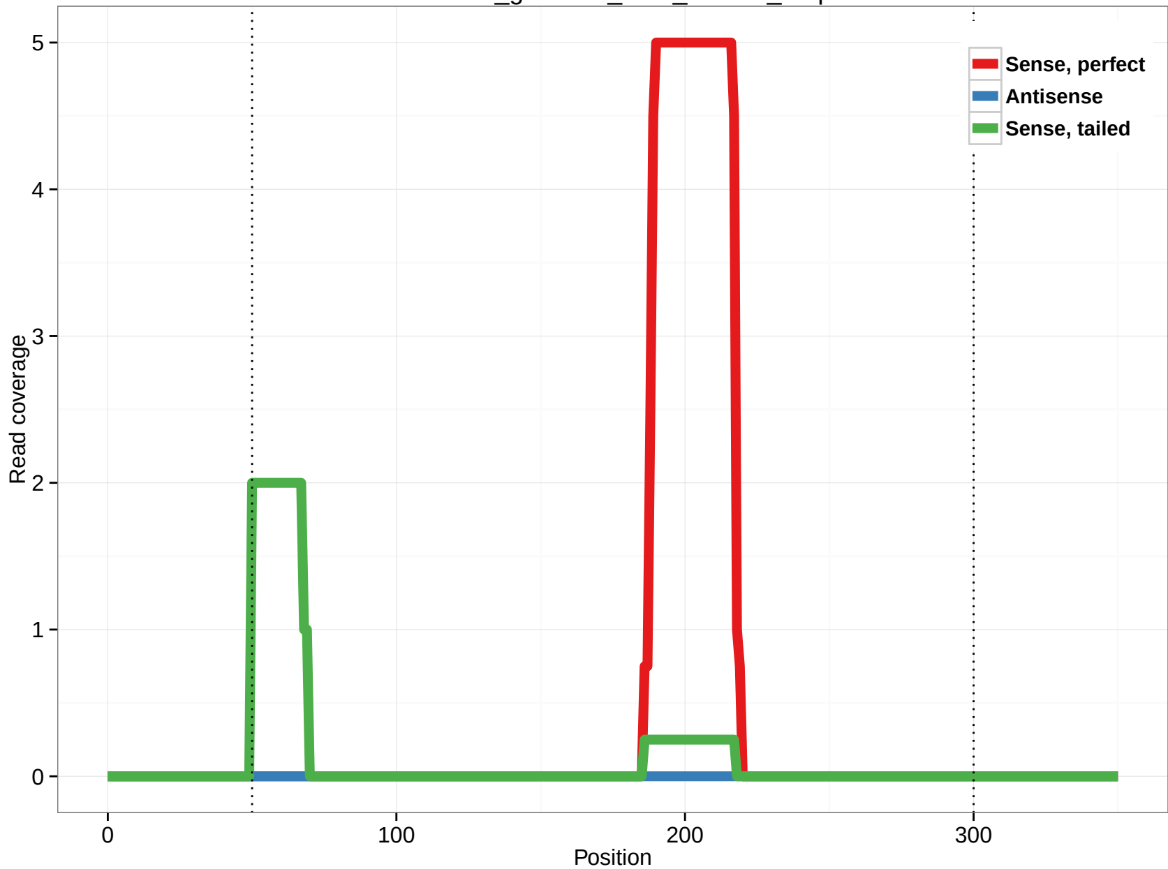
rheMac3_genscan_chr8_155.67_1.5p
