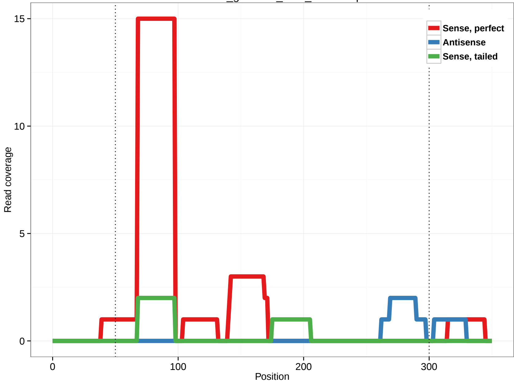
rheMac3_genscan_chr8_153.37.5p
