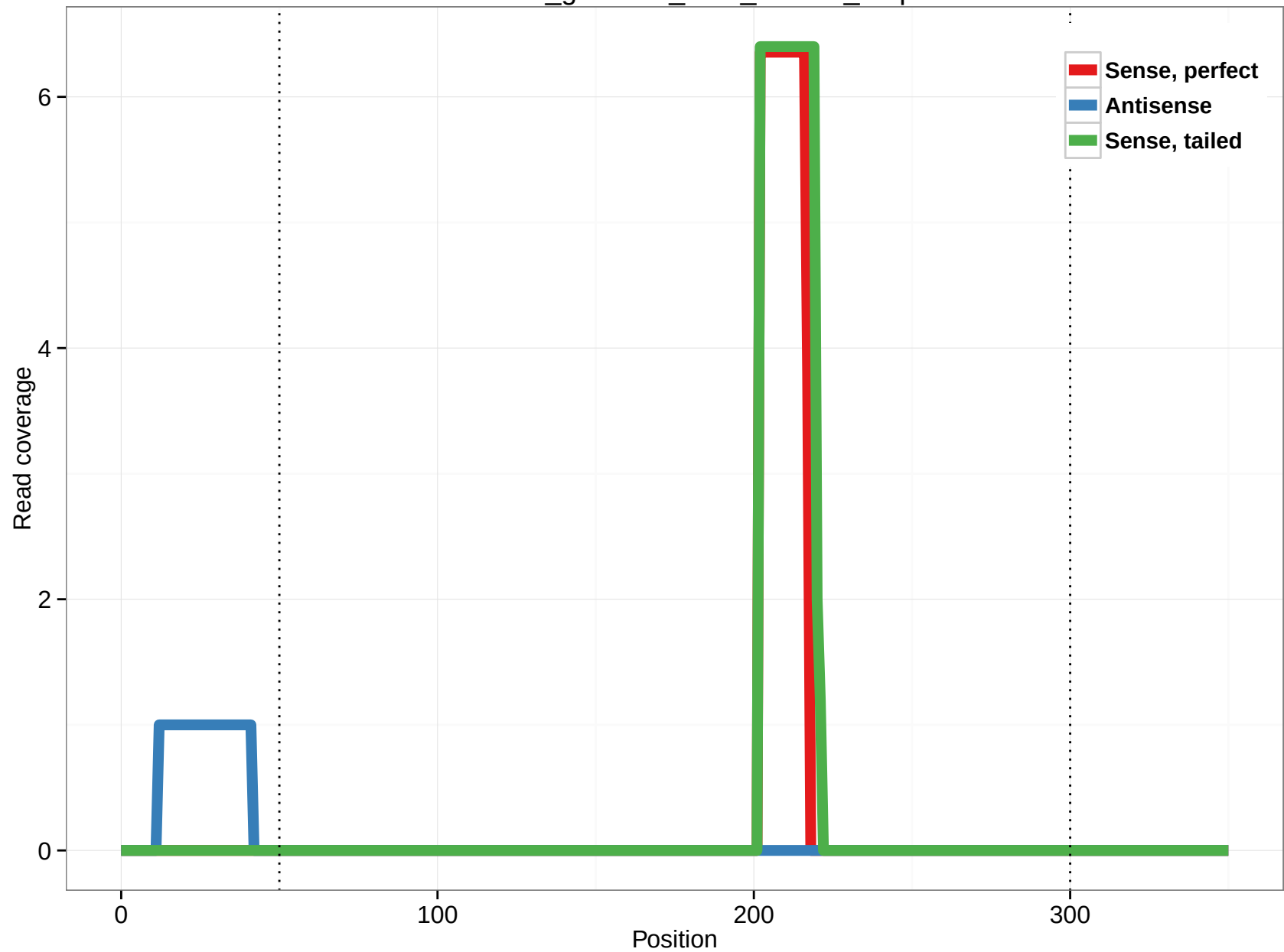
rheMac3_genscan_chr8_153.36_1.3p
