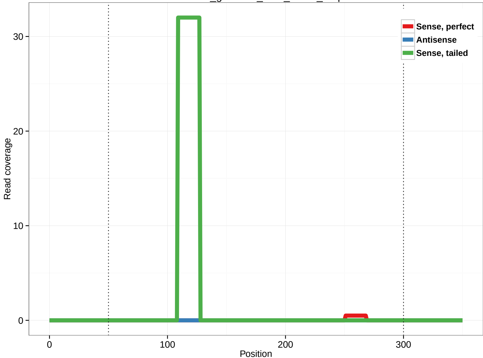
rheMac3_genscan_chr8_152.6_0.3p
