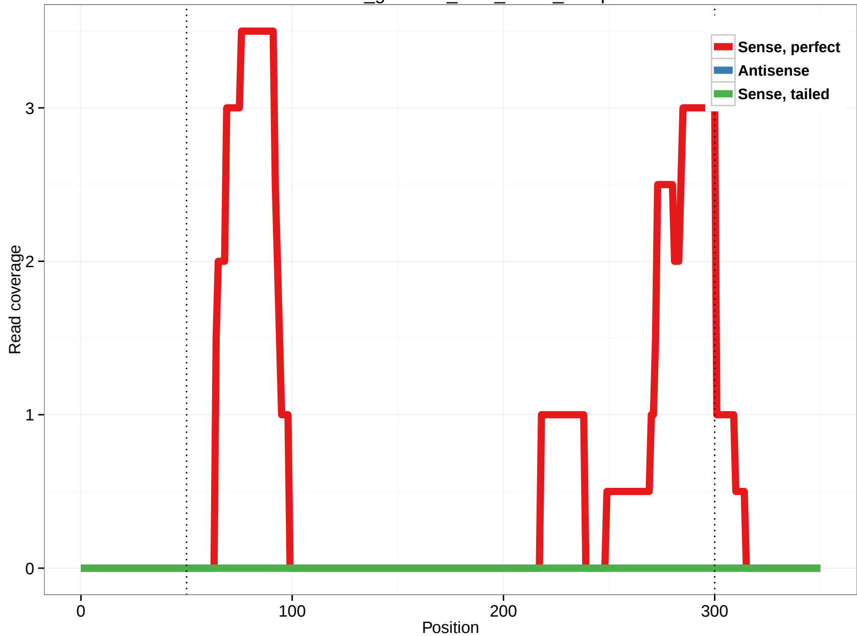
rheMac3_genscan_chr8_148.3_16.5p
