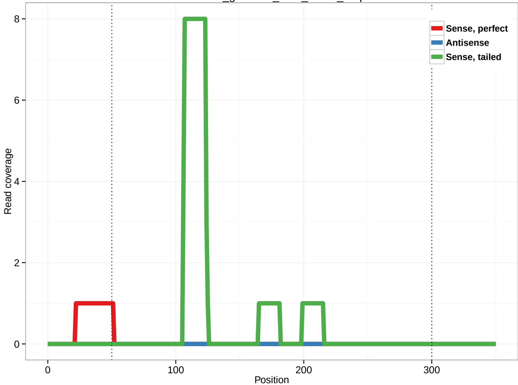
rheMac3_genscan_chr8_146.4_2.3p
