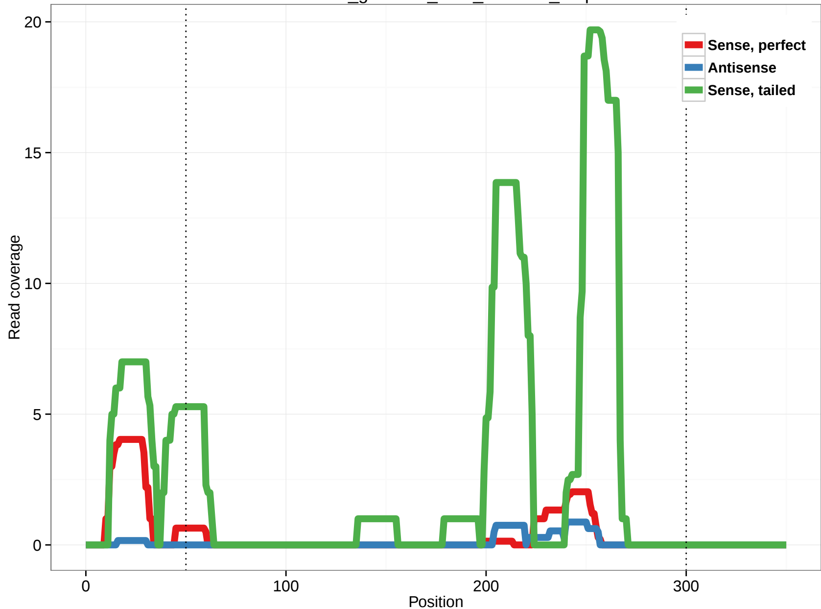
rheMac3_genscan_chr8_144.102_0.5p
