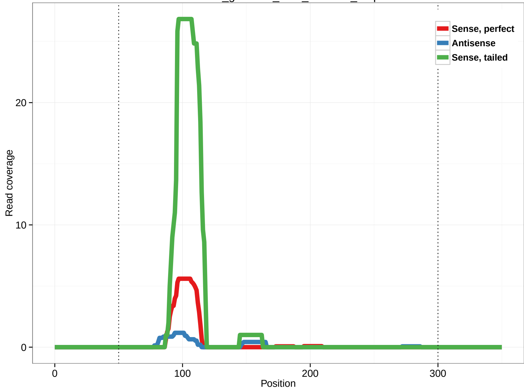
rheMac3_genscan_chr8_144.100_1.3p
