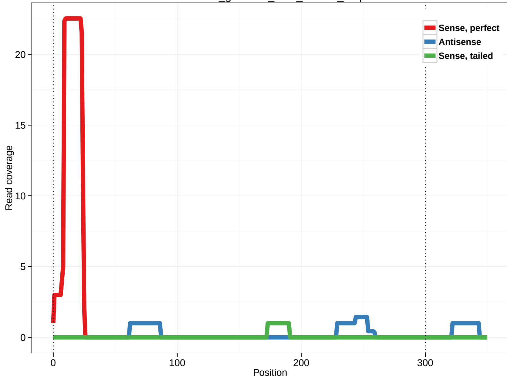
rheMac3_genscan_chr8_142.85_1.3p
