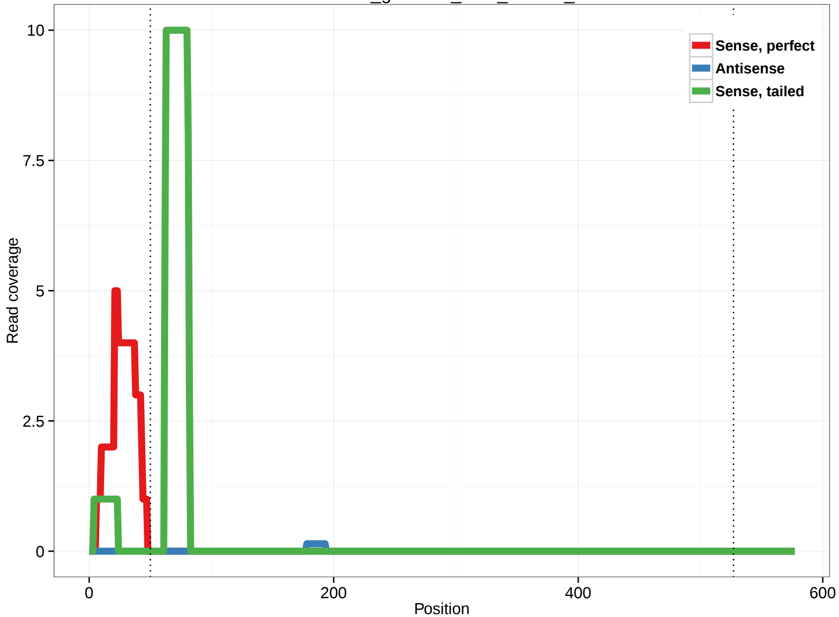
rheMac3_genscan_chr8_142.48_7
