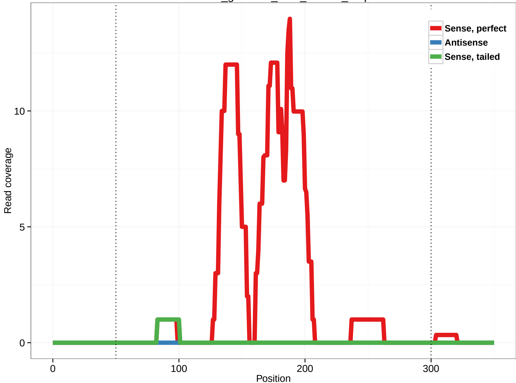
rheMac3_genscan_chr8_142.35_1.5p
