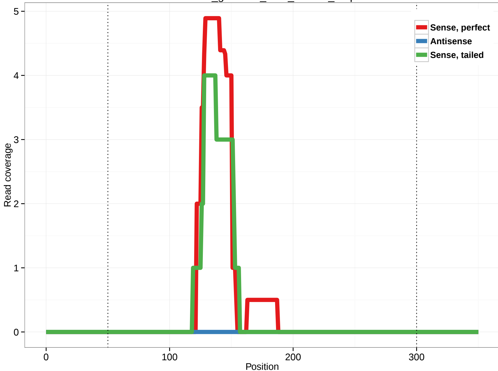
rheMac3_genscan_chr8_142.33_0.5p
