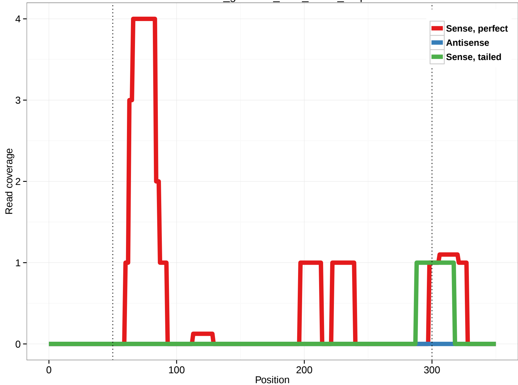
rheMac3_genscan_chr8_141.7_3.3p
