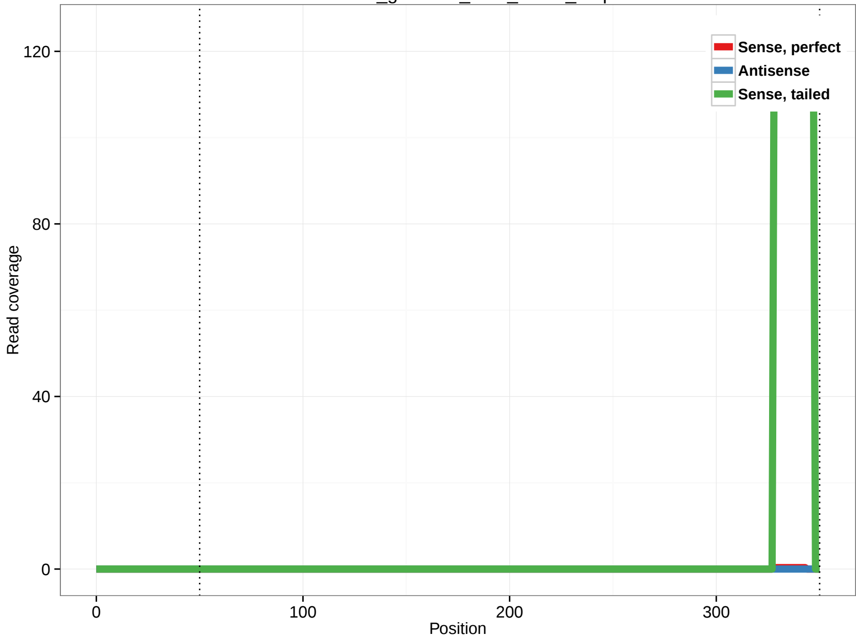
rheMac3_genscan_chr8_140.7_6.5p
