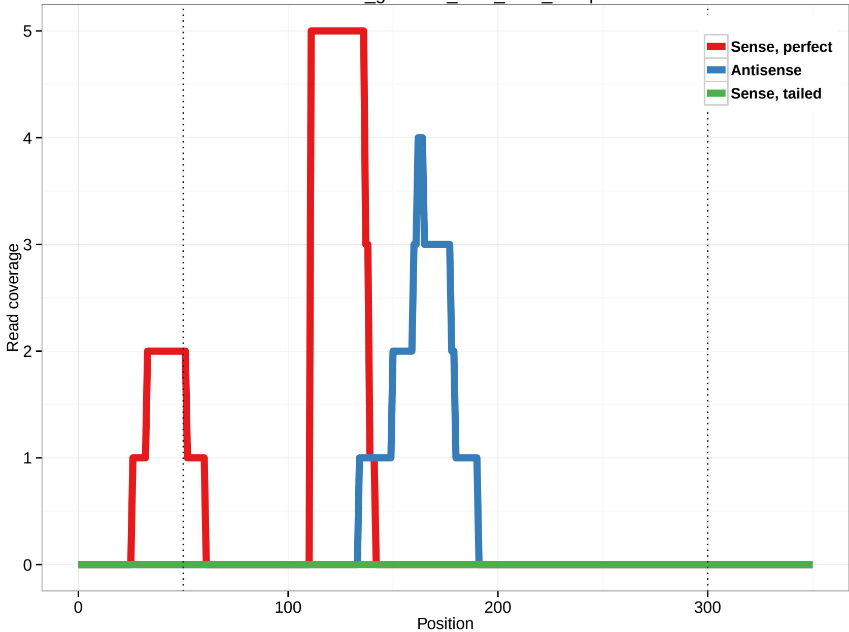
rheMac3_genscan_chr8_13.3_14.3p
