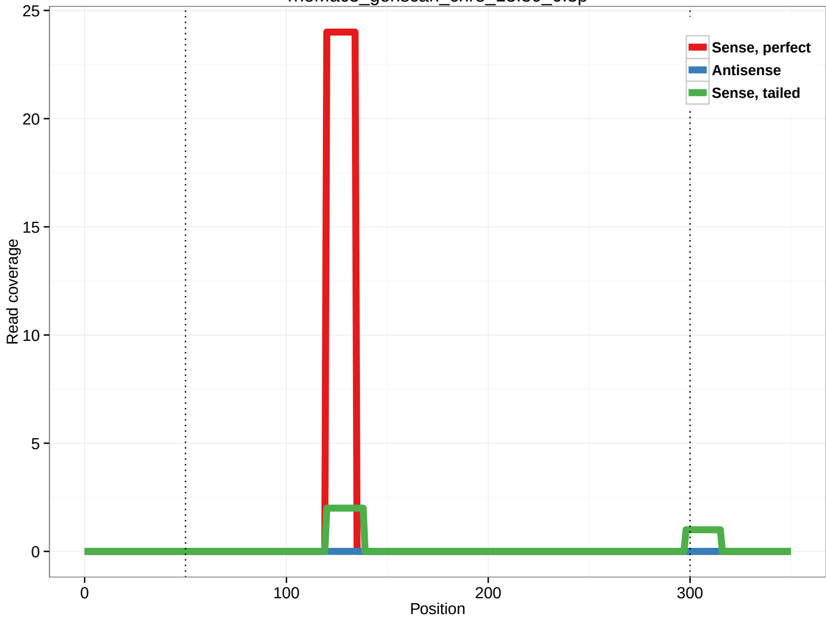
rheMac3_genscan_chr8_13.30_0.3p
