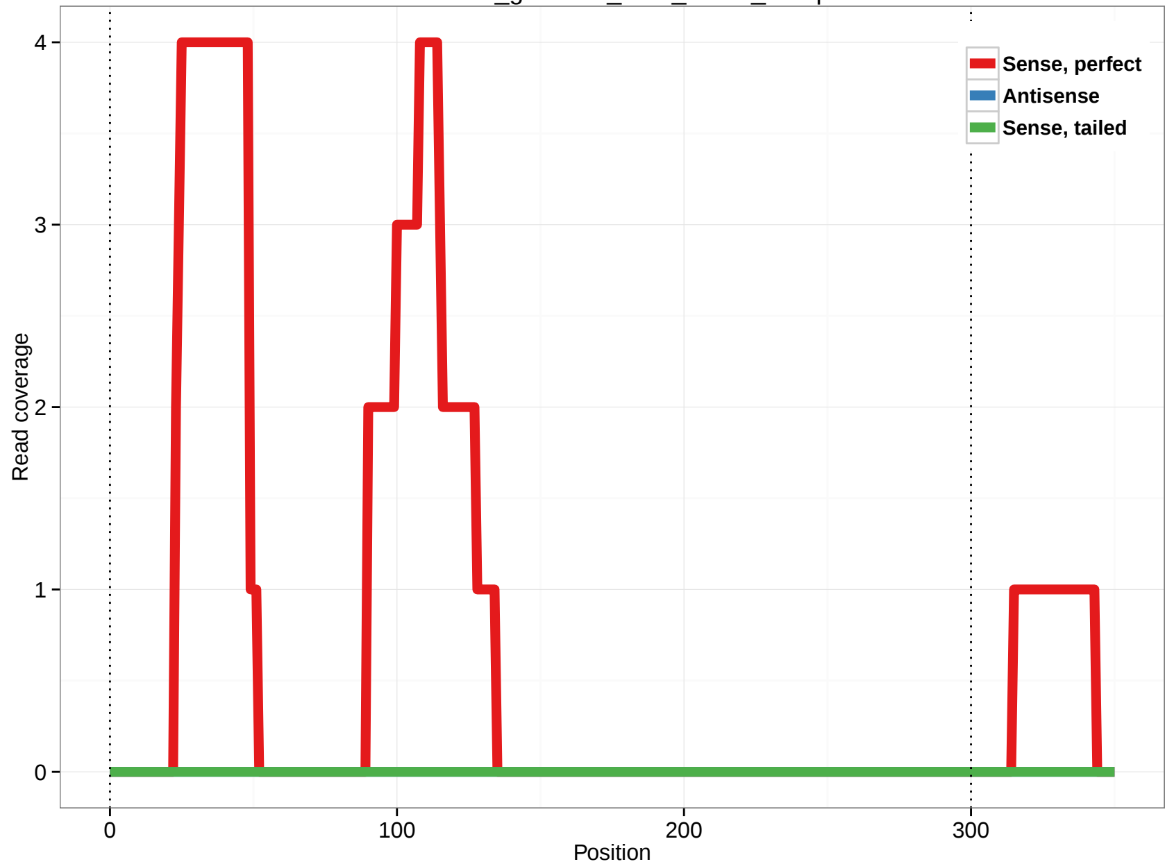
rheMac3_genscan_chr8_13.12_16.3p
