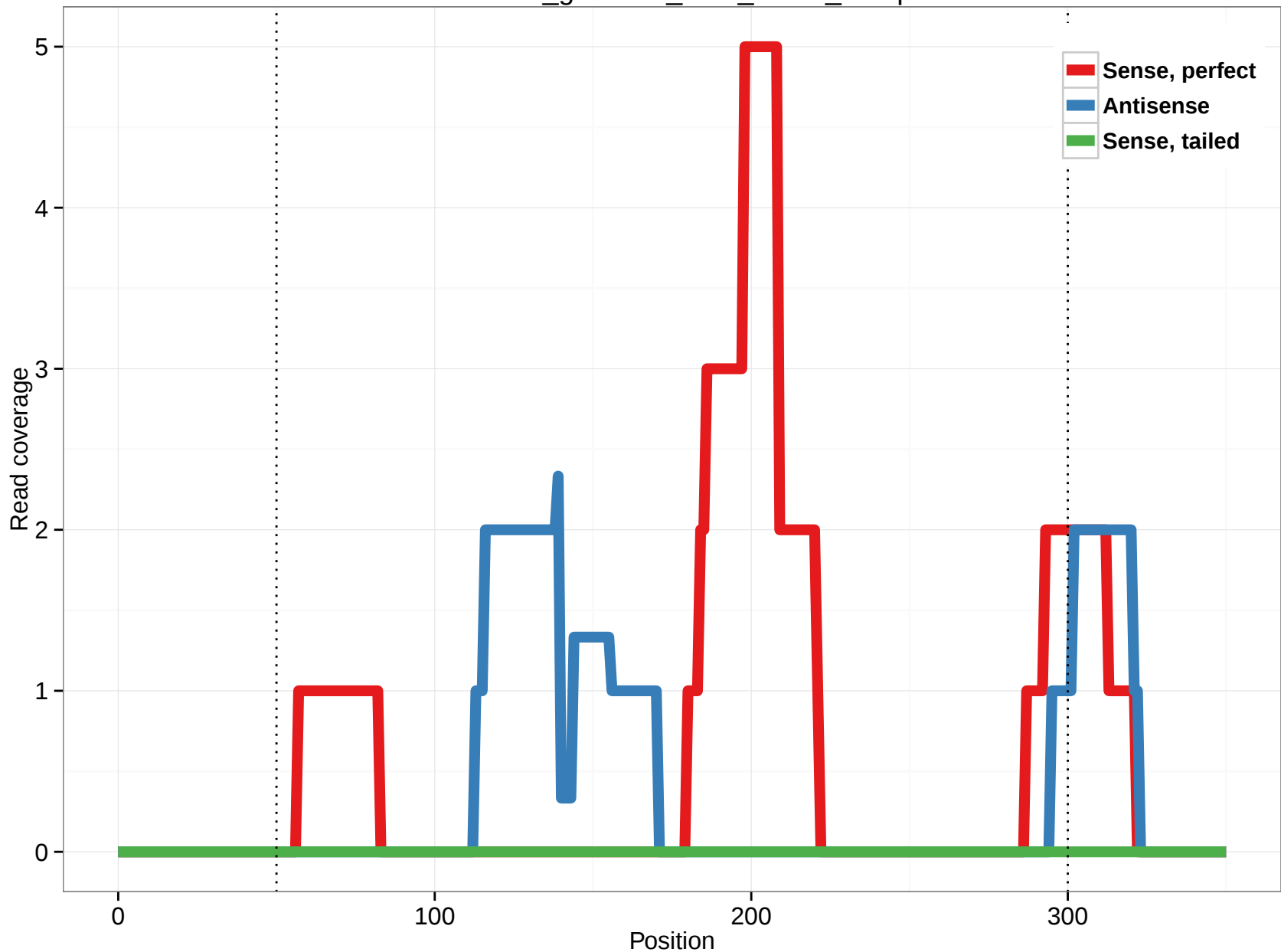
rheMac3_genscan_chr8_13.10_22.3p
