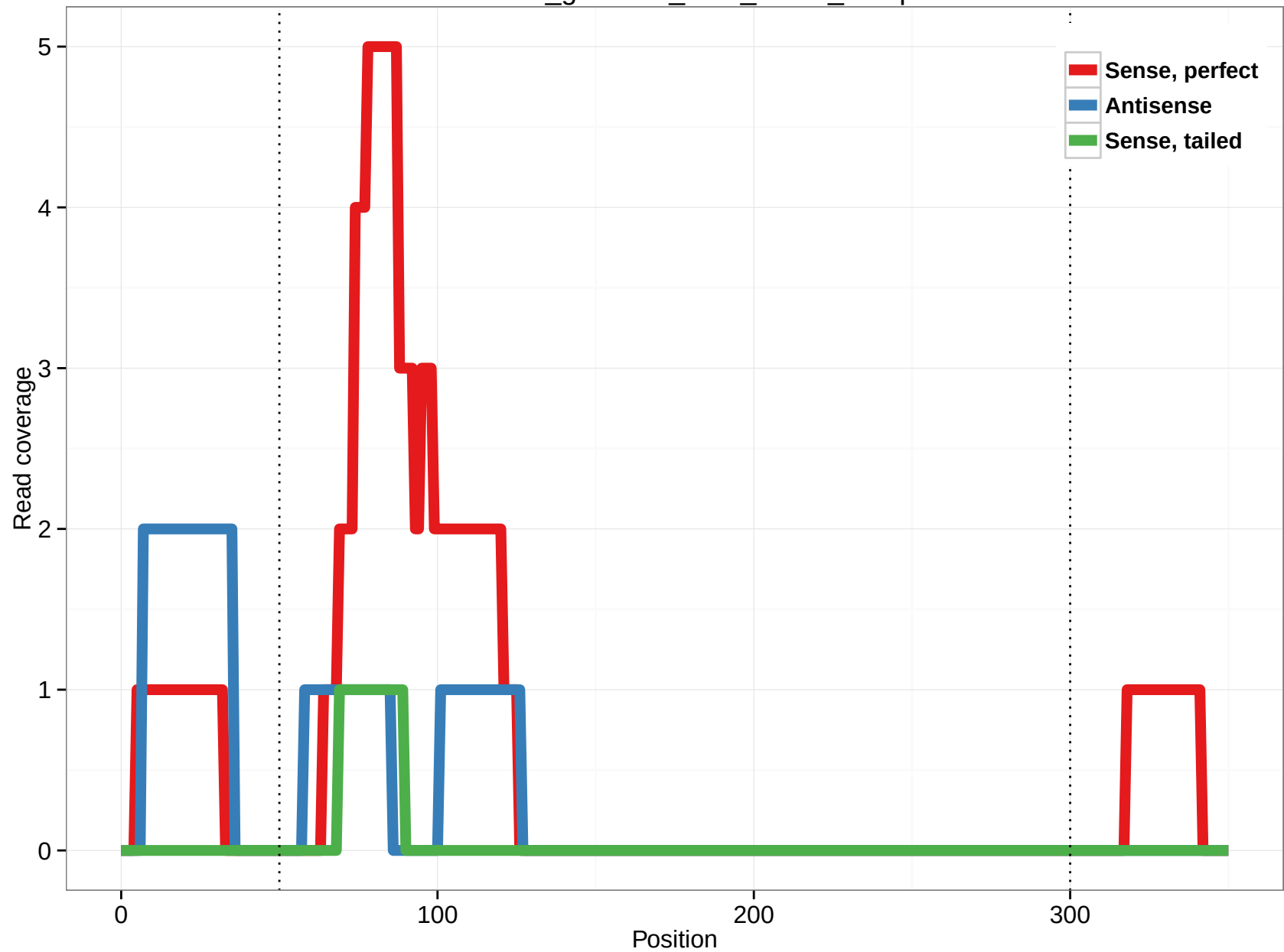
rheMac3_genscan_chr8_13.10_14.3p
