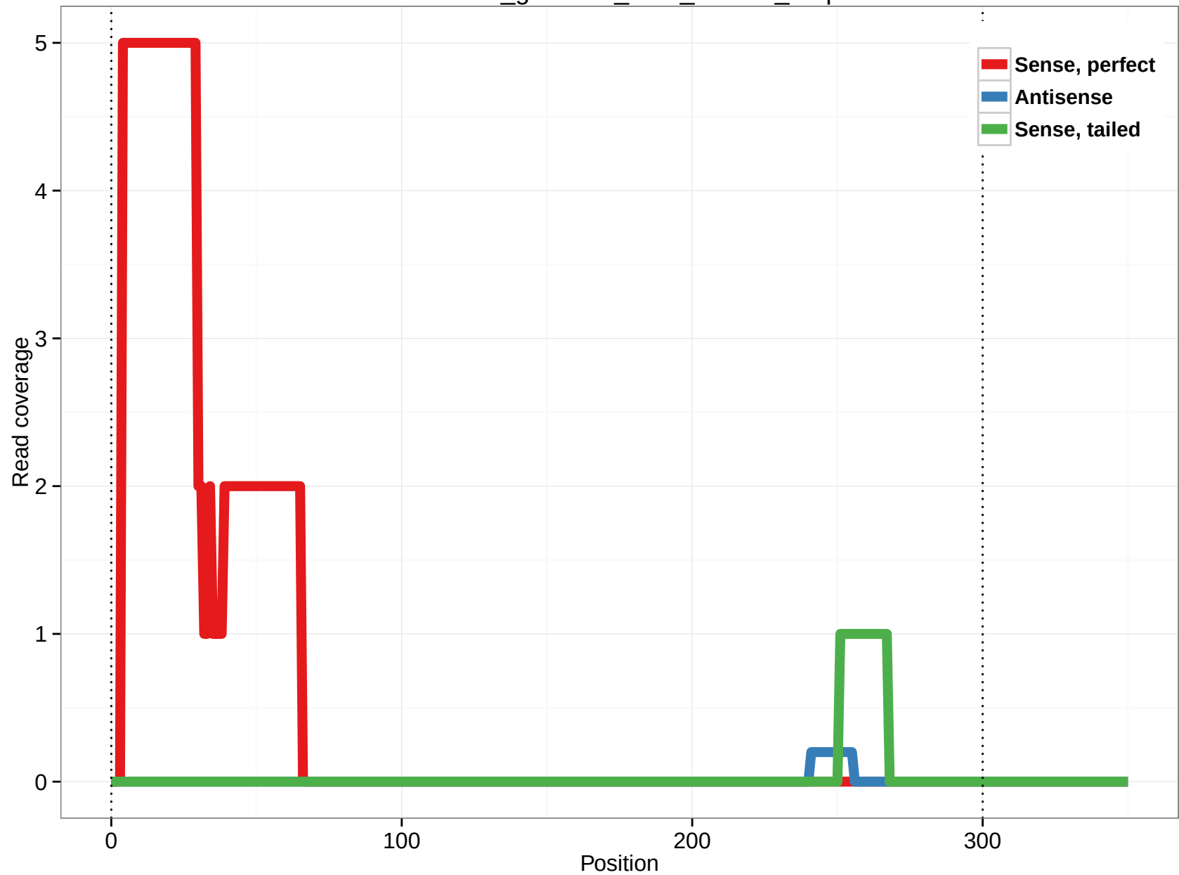
rheMac3_genscan_chr8_122.94_9.3p
