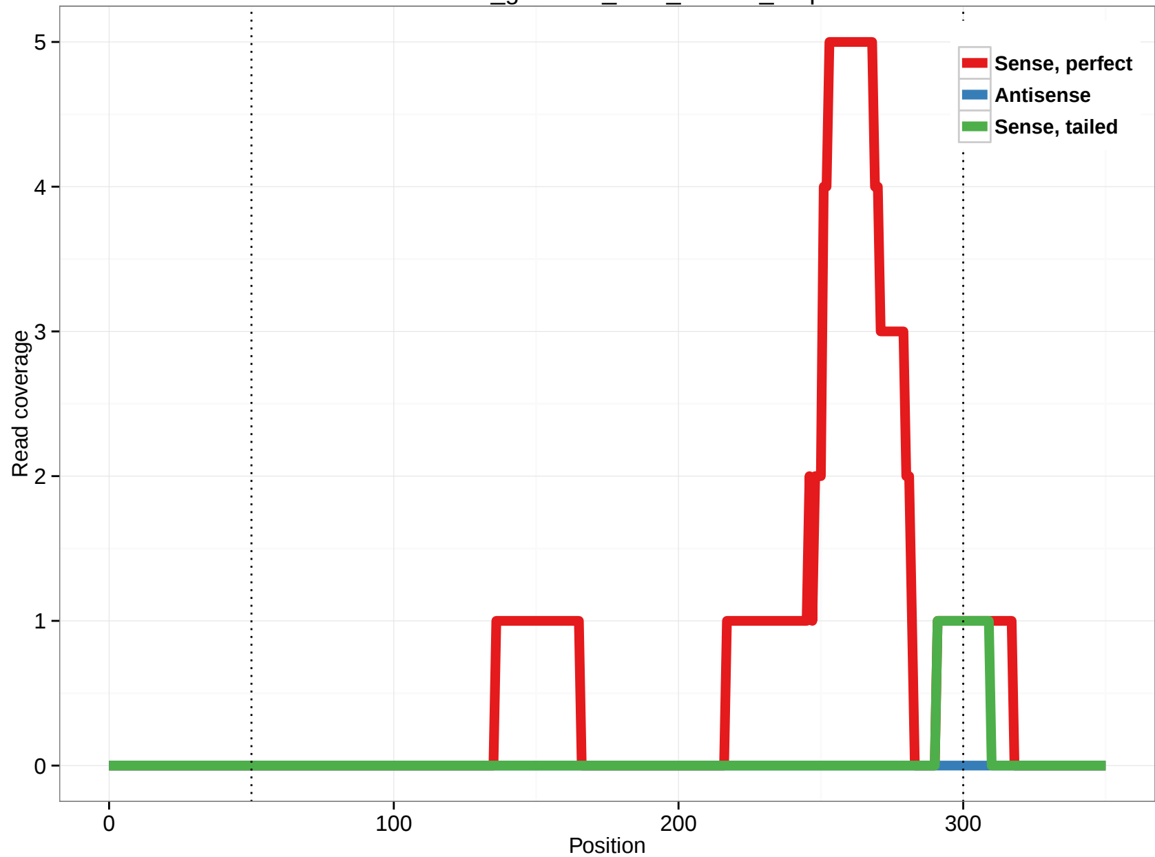
rheMac3_genscan_chr8_122.59_7.3p
