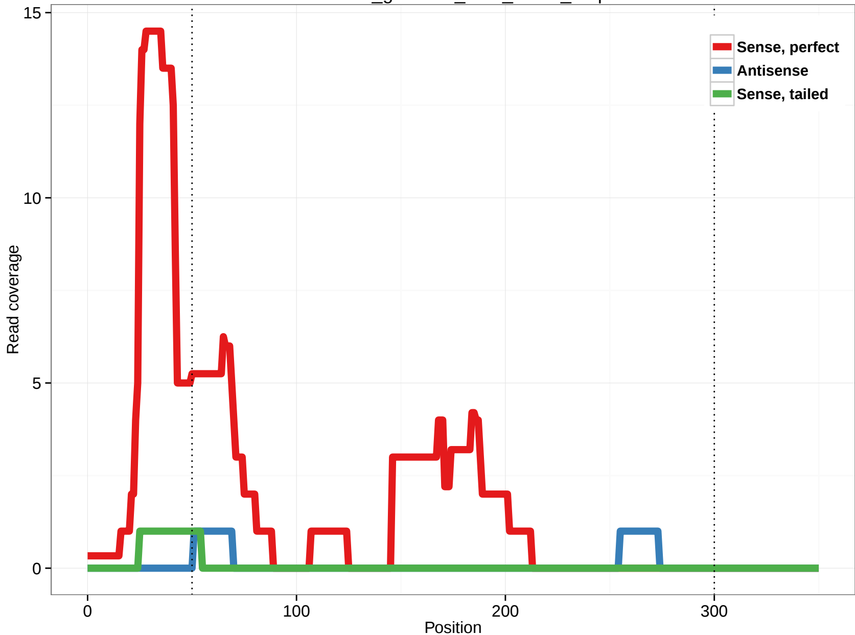
rheMac3_genscan_chr8_119.6_3.3p
