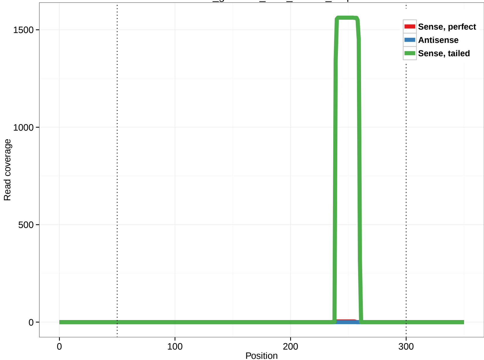
rheMac3_genscan_chr8_119.33_5.5p
