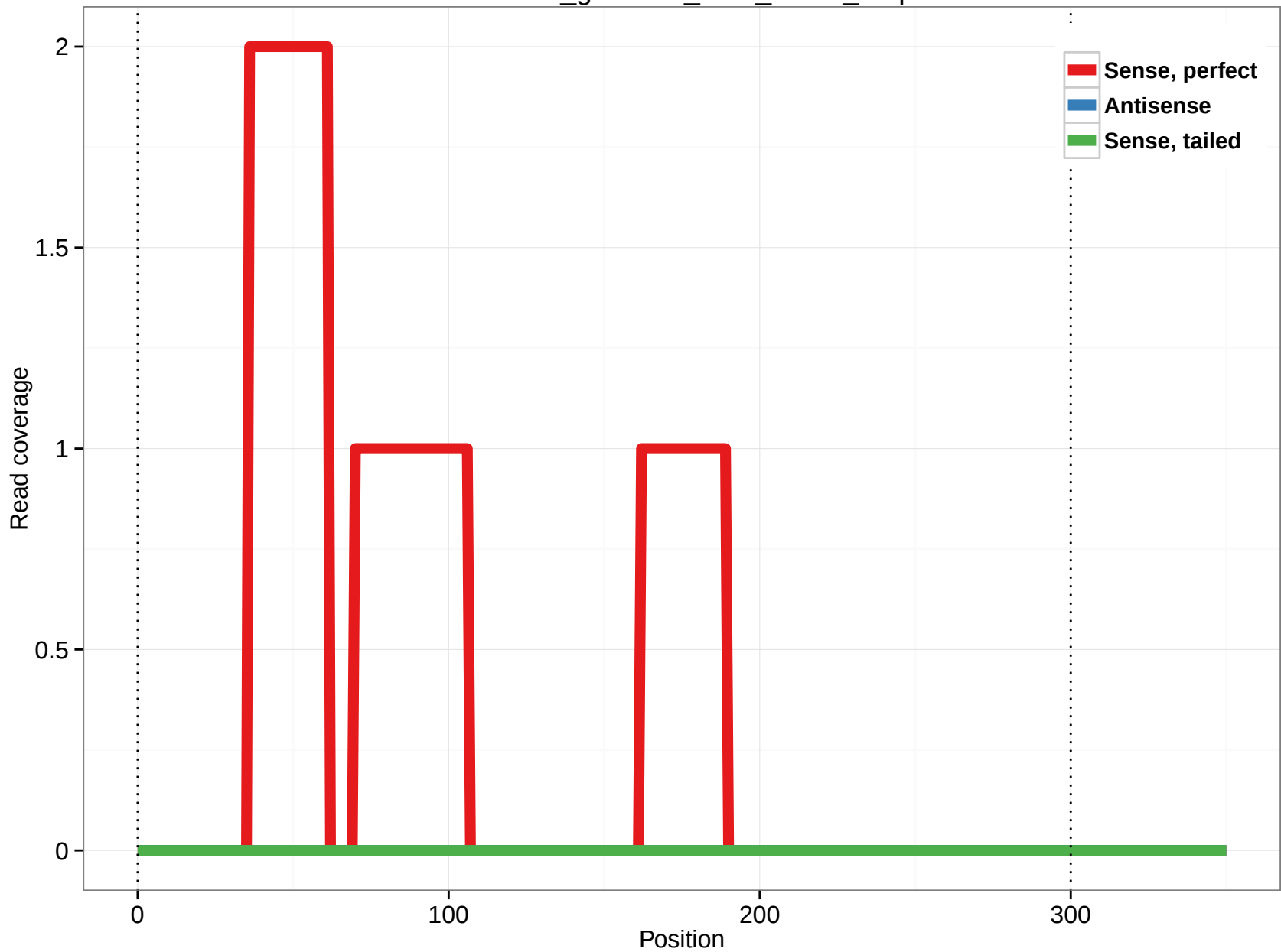
rheMac3_genscan_chr8_114.9_7.3p
