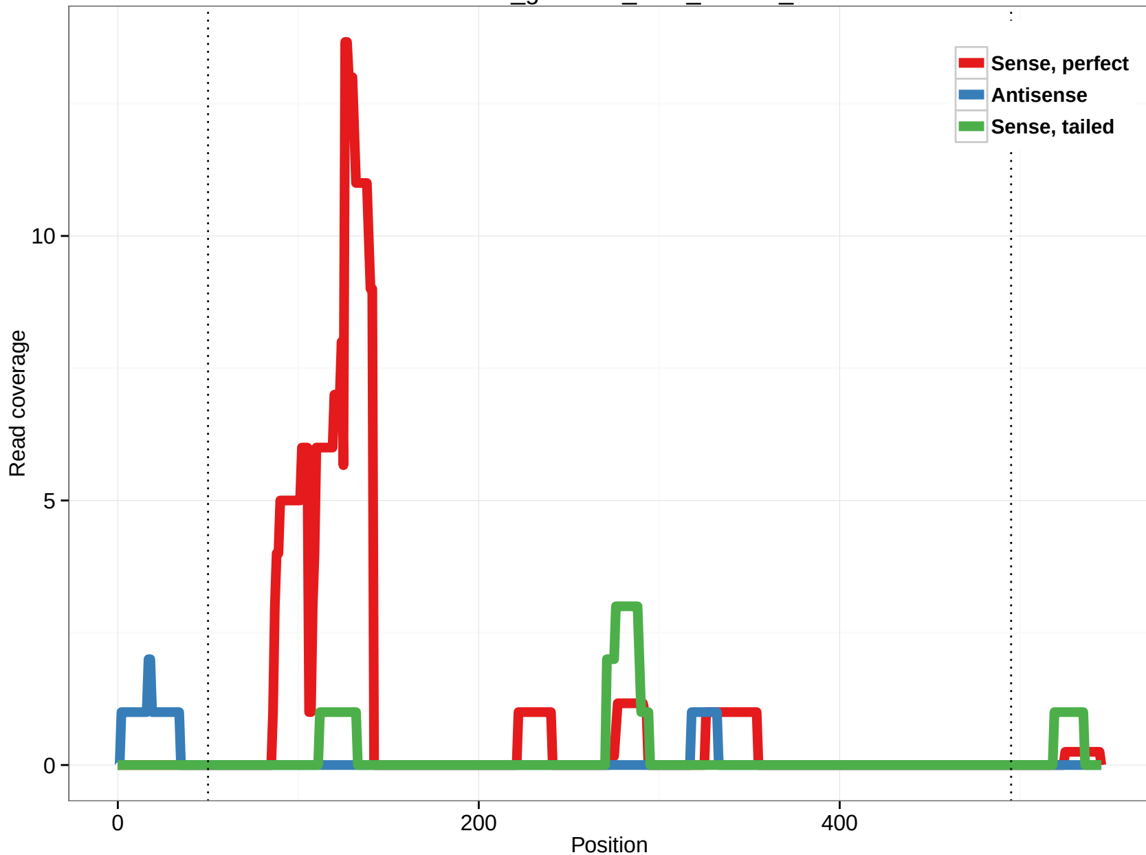
rheMac3_genscan_chr8_111.46_0
