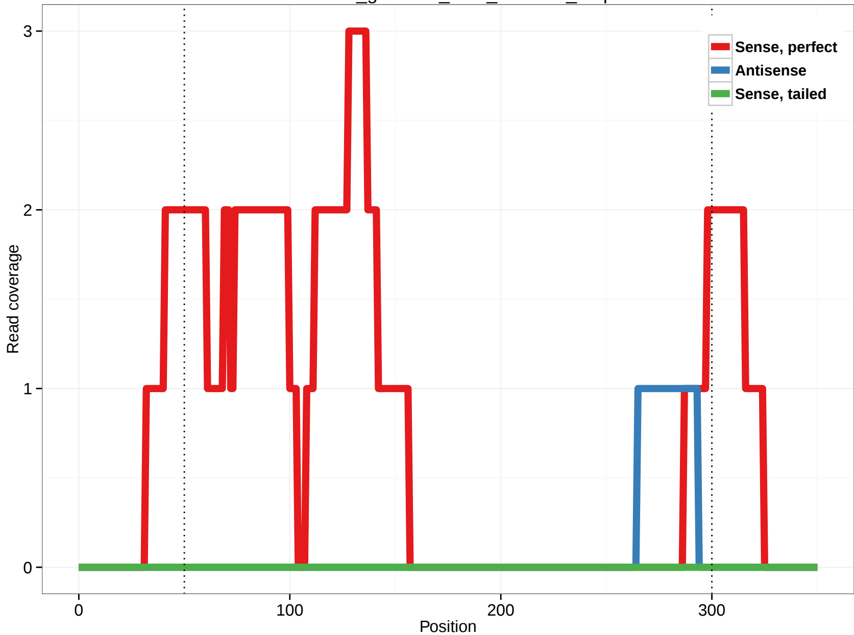
rheMac3_genscan_chr8_111.138_0.3p
