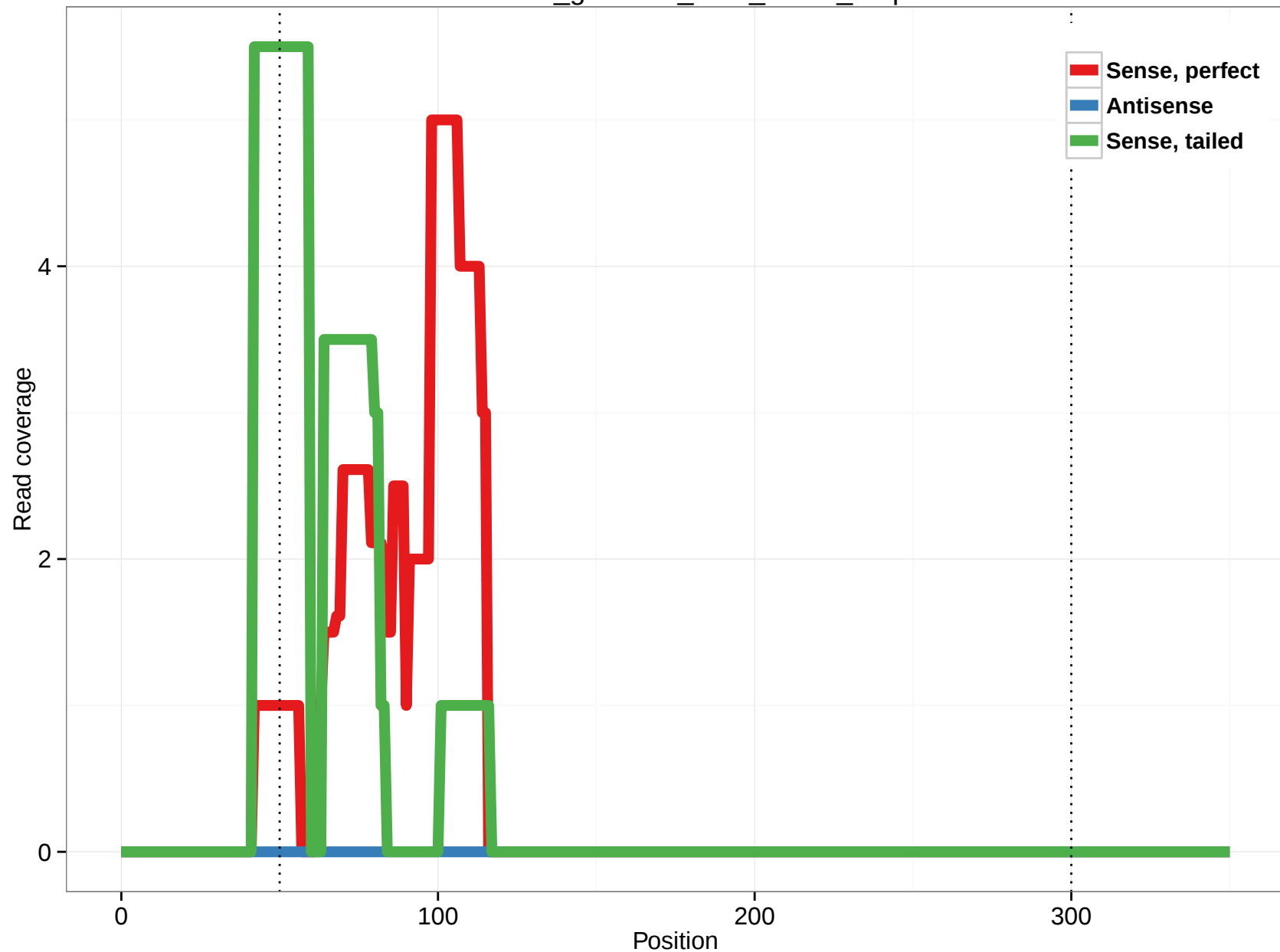
rheMac3_genscan_chr8_102.8_0.5p
