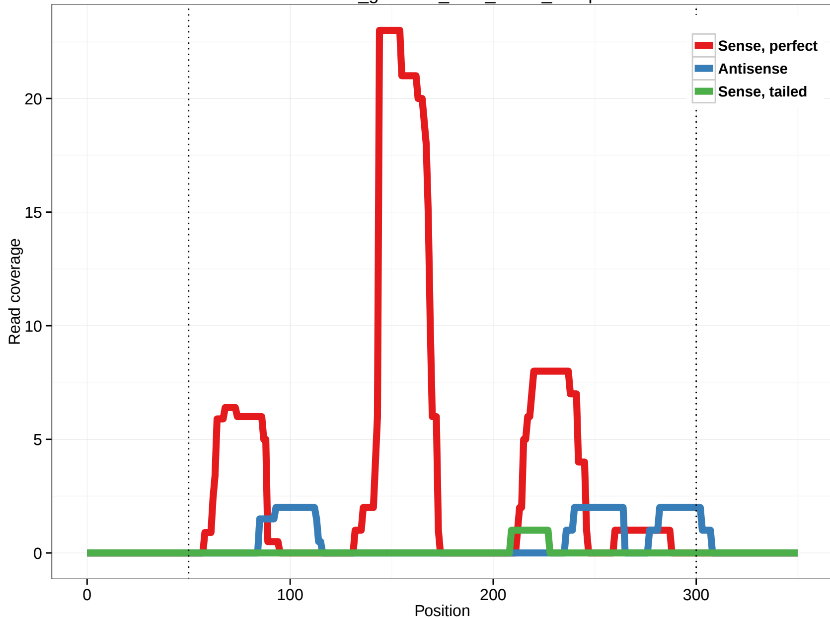
rheMac3_genscan_chr8_102.4_20.5p
