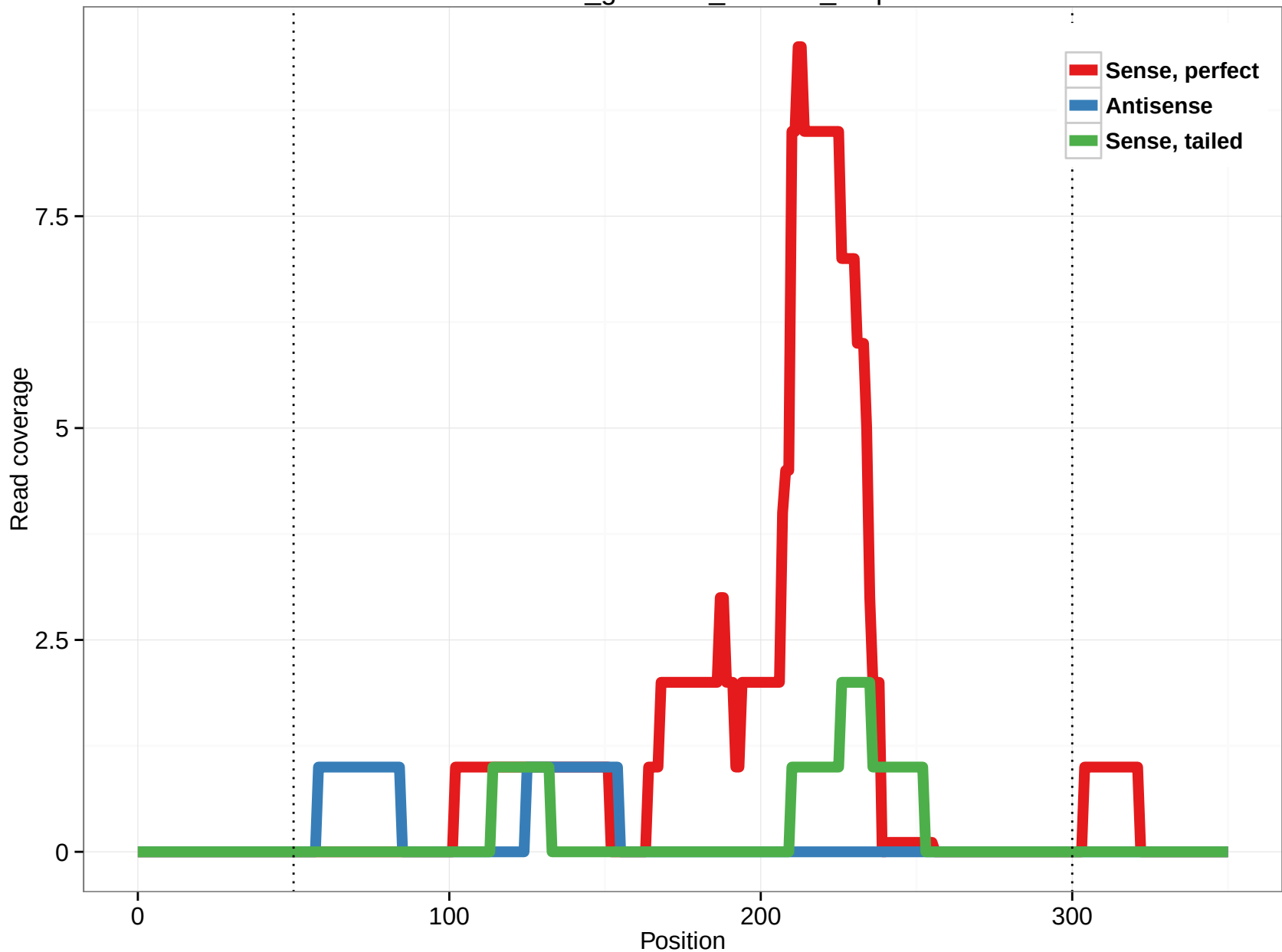
rheMac3_genscan_chr7.99_3.5p
