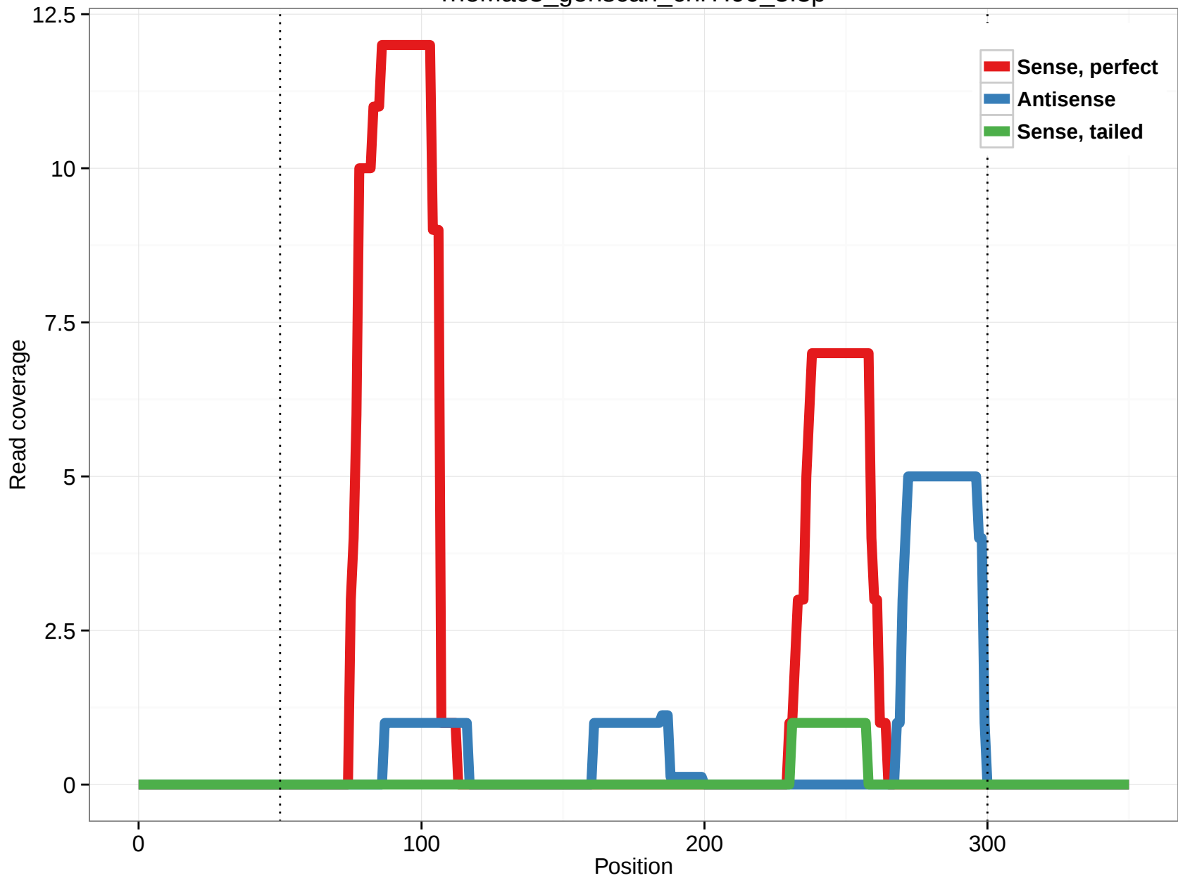
rheMac3_genscan_chr7.99_3.3p
