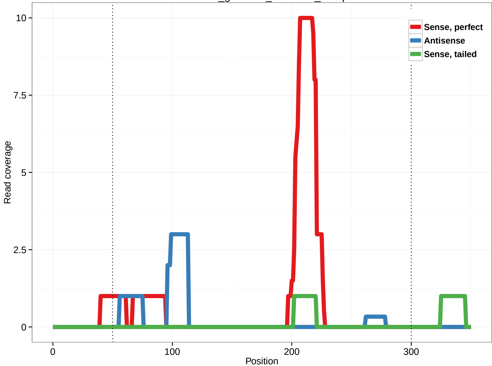
rheMac3_genscan_chr7.996_27.3p
