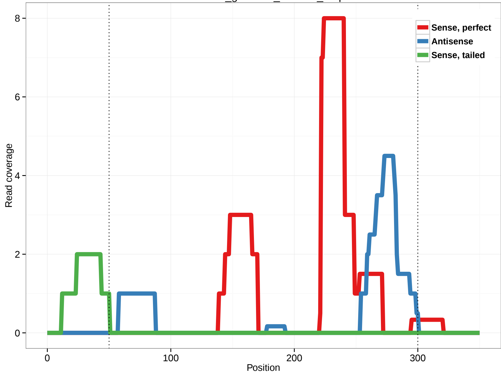
rheMac3_genscan_chr7.97_3.3p
