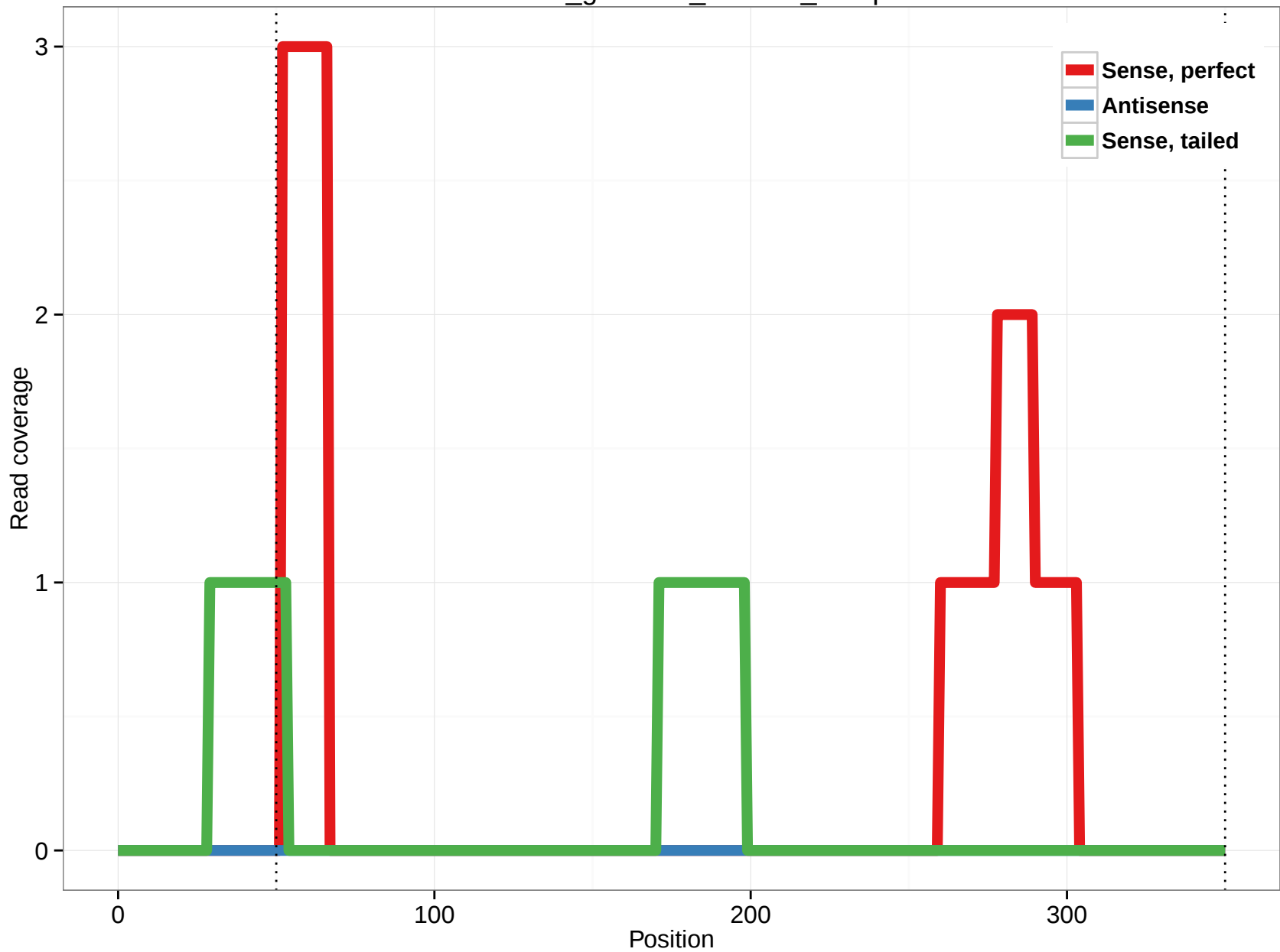
rheMac3_genscan_chr7.96_13.5p
