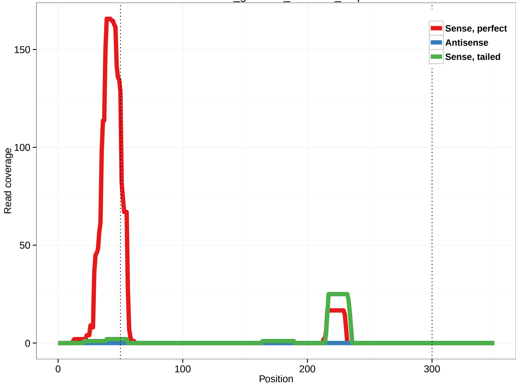
rheMac3_genscan_chr7.969_0.5p
