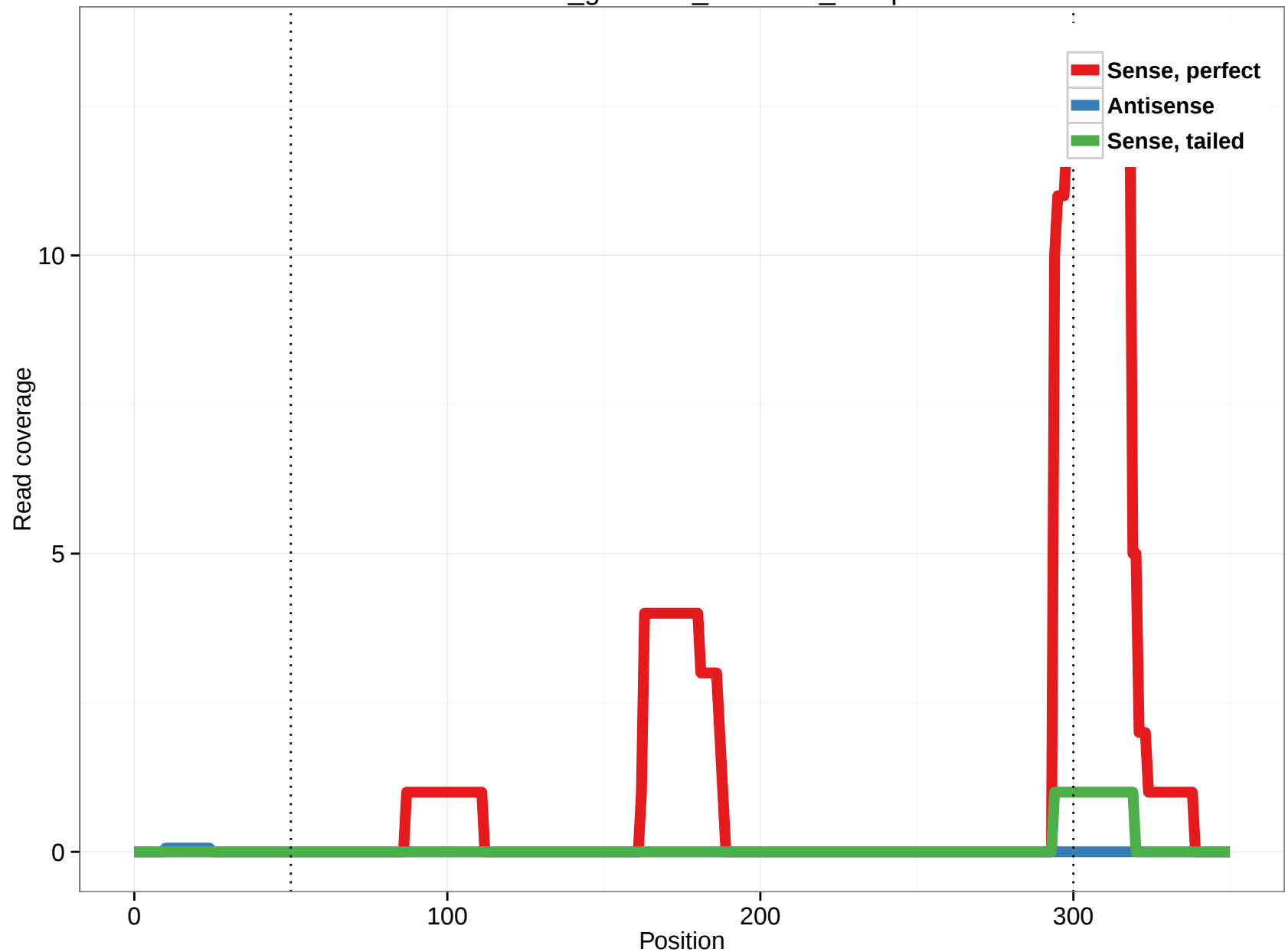
rheMac3_genscan_chr7.963_12.3p
