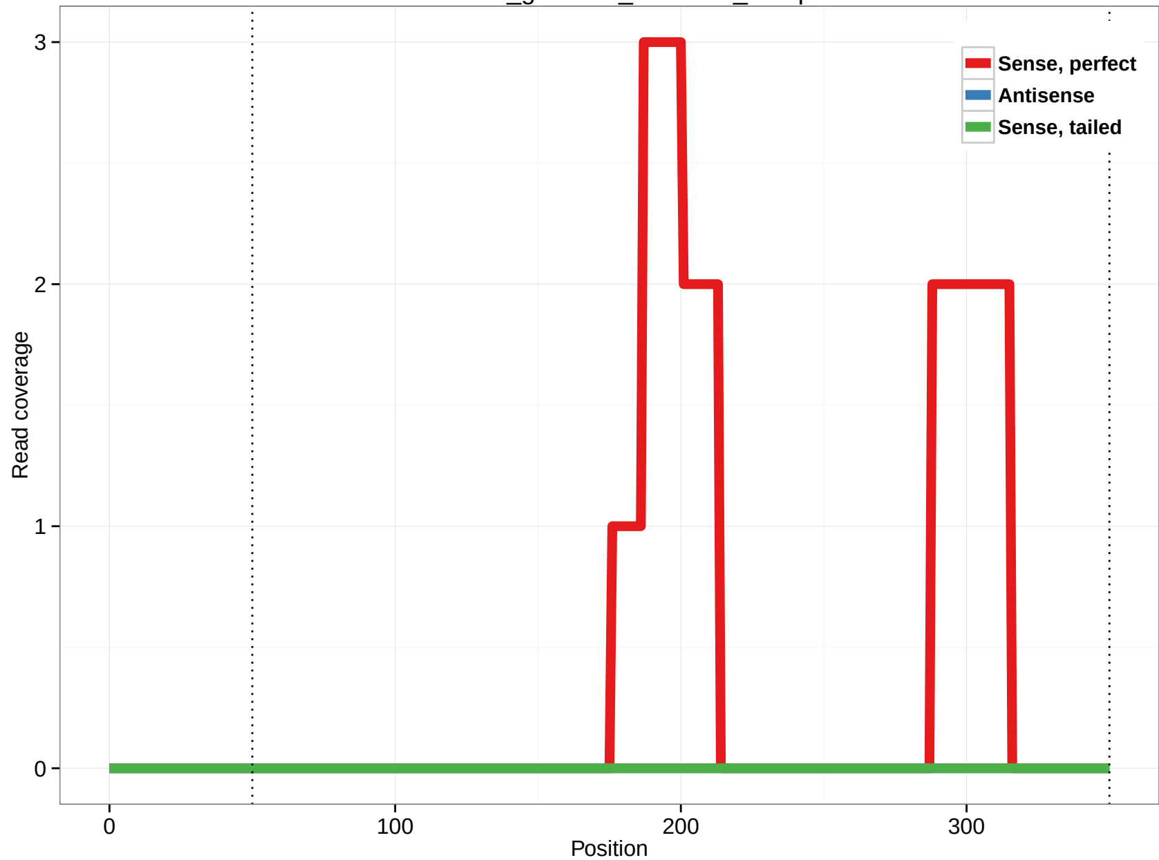
rheMac3_genscan_chr7.963_11.5p
